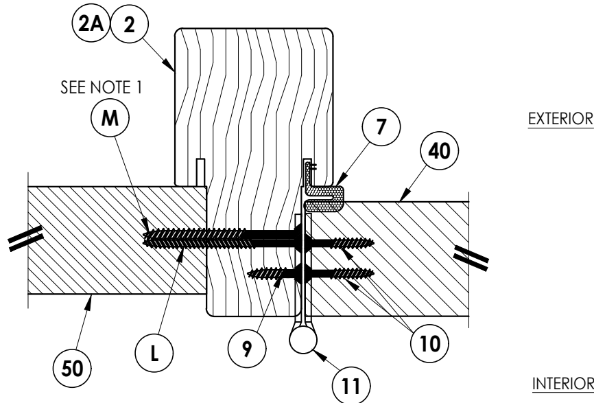
4 7 HORIZONTAL CROSS SECTION Inswing shown (Outswing similar)
